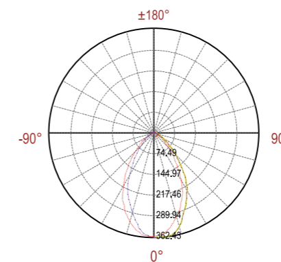
Light intensity distribution curve
