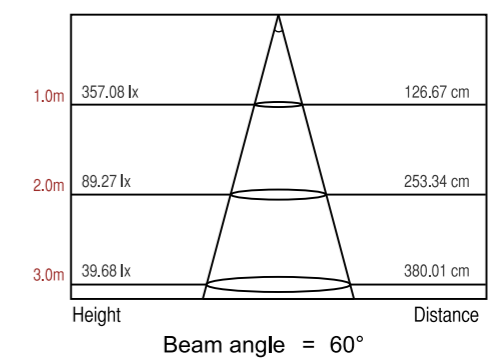
Light intensity distribution curve
